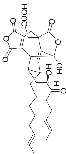
phomoidride C (3)
