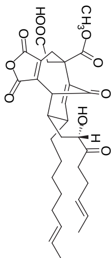
methyl ester 5
